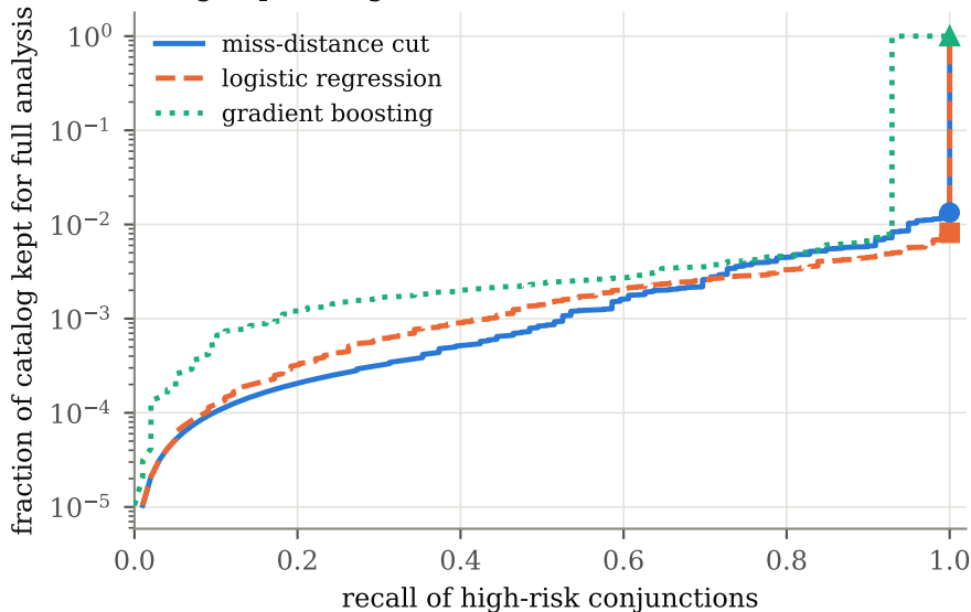
Triage operating curves (lower is better)
