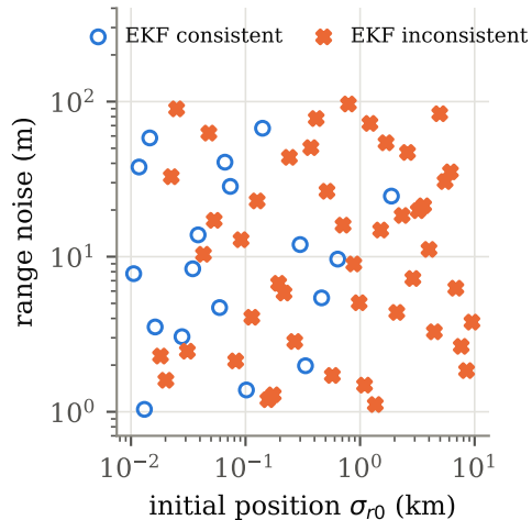
(c) where the EKF fails
