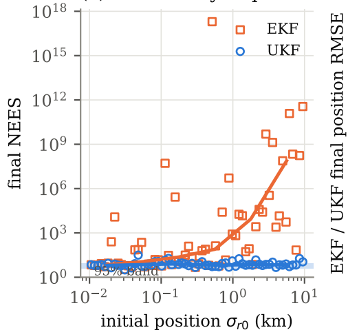
(a) consistency vs prior width
