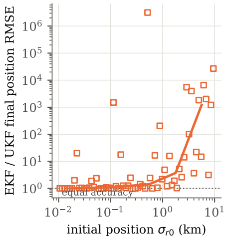
(b) accuracy penalty
