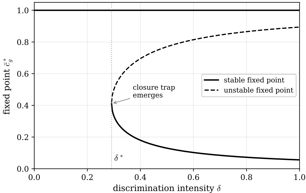
Closure as \delta increases ( \tilde{\gamma}=0.05 , \mu=0.05 )
