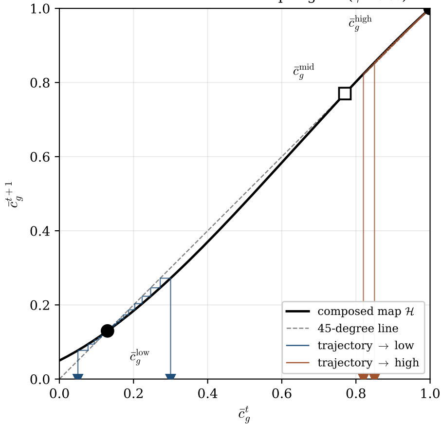
Cobweb iteration in the trap regime ( \tilde{\gamma} = 0.05 )
