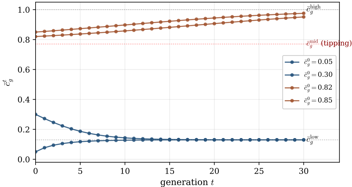
Group-prior trajectories across generations ( \tilde{\gamma} = 0.05 )
