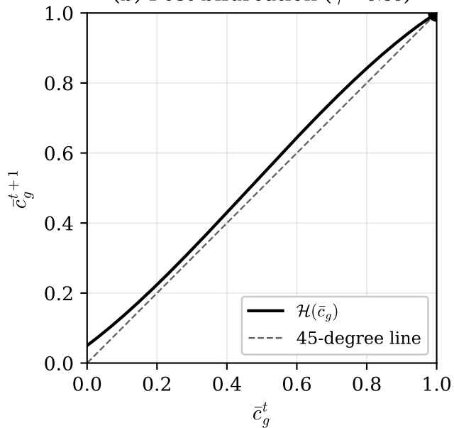
(b) Post-bifurcation ( \tilde{\gamma} = 0.30 )
