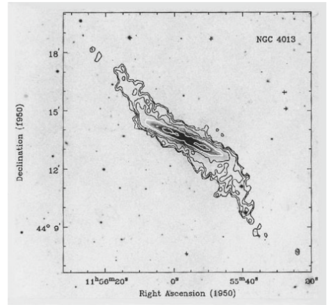
Figure 2.6: Edge-on spiral NGC4013, optical emission in grey, superimposed by intensity of cold 21-cm emitting gas (HI). The warping begins only about when the visible disk ends.
