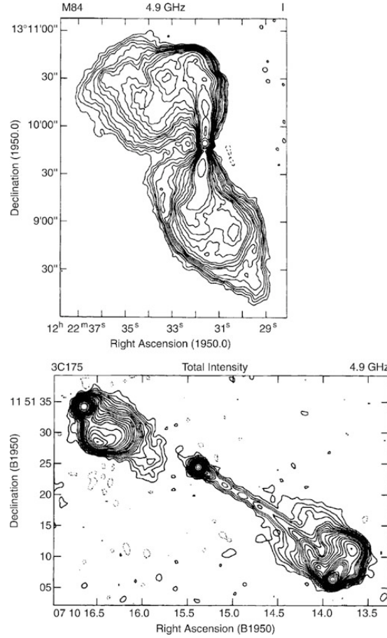
Figure 3.2: Radio galaxies M84 with FRI (top) and 3C175 with FRII (bottom) extended radio sources. Source: Ref 1
