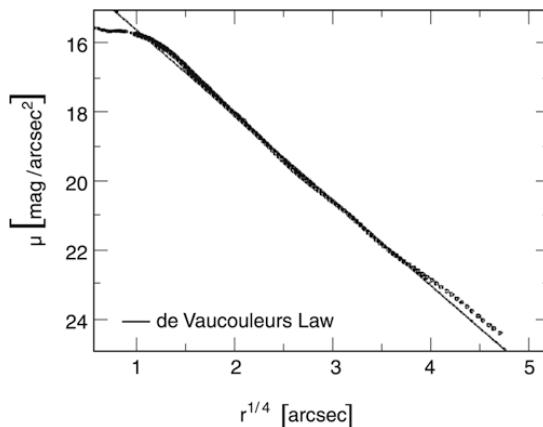
Figure 2.4: Surface brightness of galaxy NGC 4472 fitted with a de Vaucouleur's profile. It is evident that this galaxy has a core/light deficit.
