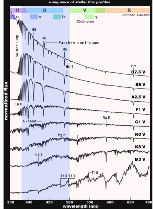
Figure 1.4: The spectra of the different spectral classes of stars.
