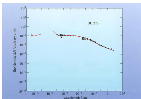
Figure 3.1: SED of an active galaxy (quasar) 3C 273. We can observe the big blue bump in the x-ray and uv regions. Source: Ref. 2
