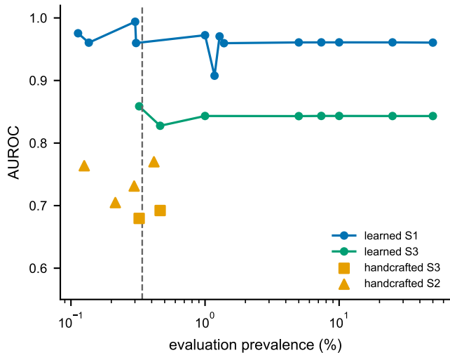
(a) AUROC
