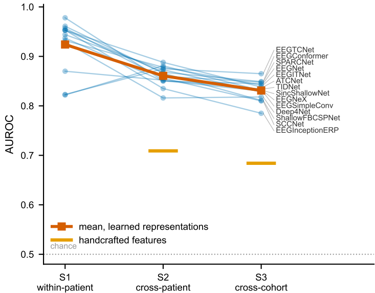
(a) generalisation by setting
