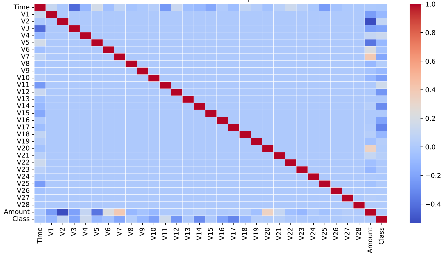
Correlation Heatmap
