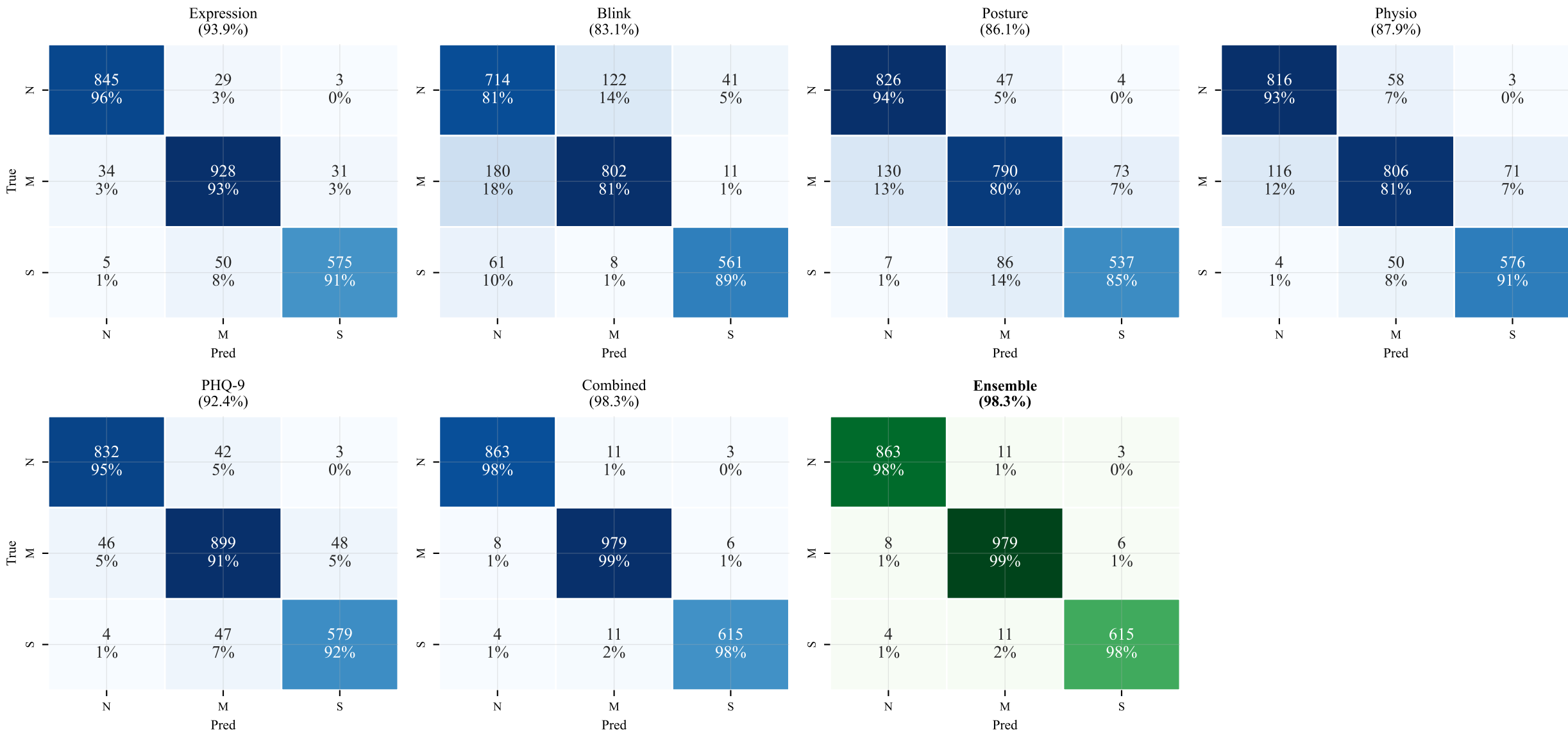
Fig. 11: Confusion Matrices for All Models
