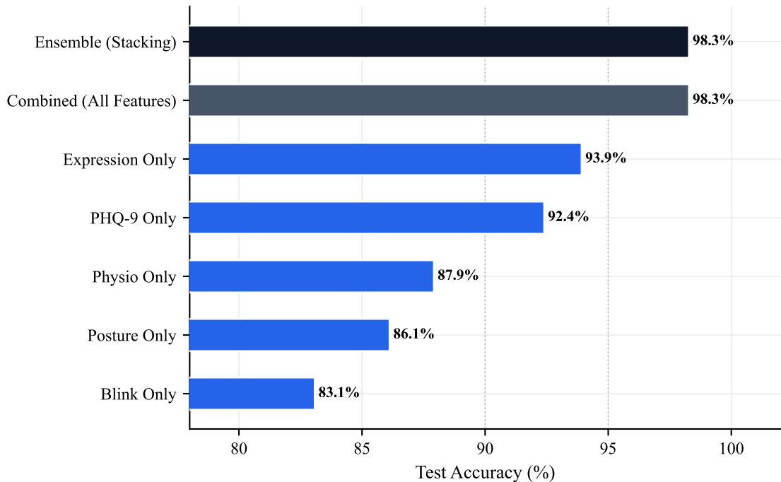
Fig. 12: Ablation Study — Single Modality vs. Fusion
