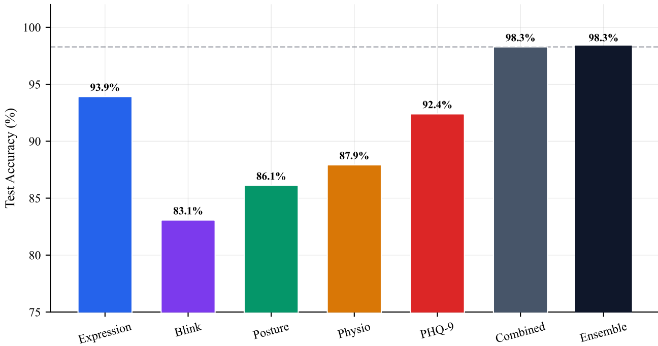
Fig. 1: Comparative Model Accuracy on Held-Out Test Set
