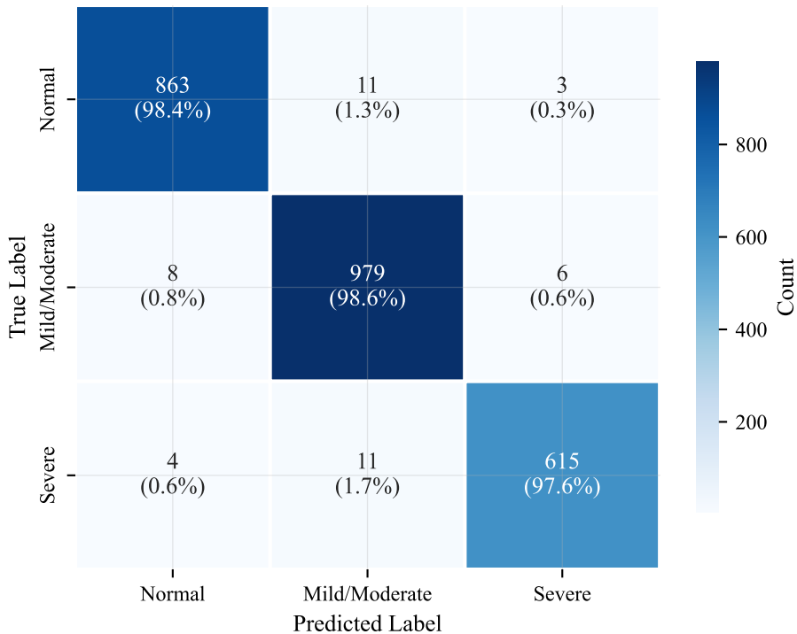
Fig. 2: Confusion Matrix — Stacking Ensemble
