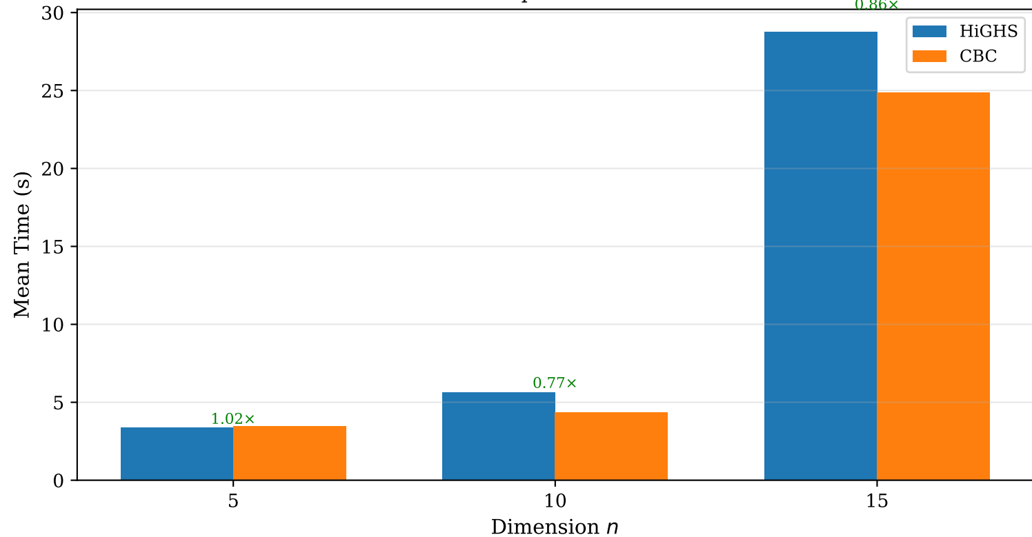
MILP Solver Comparison: HiGHS vs. CBC
