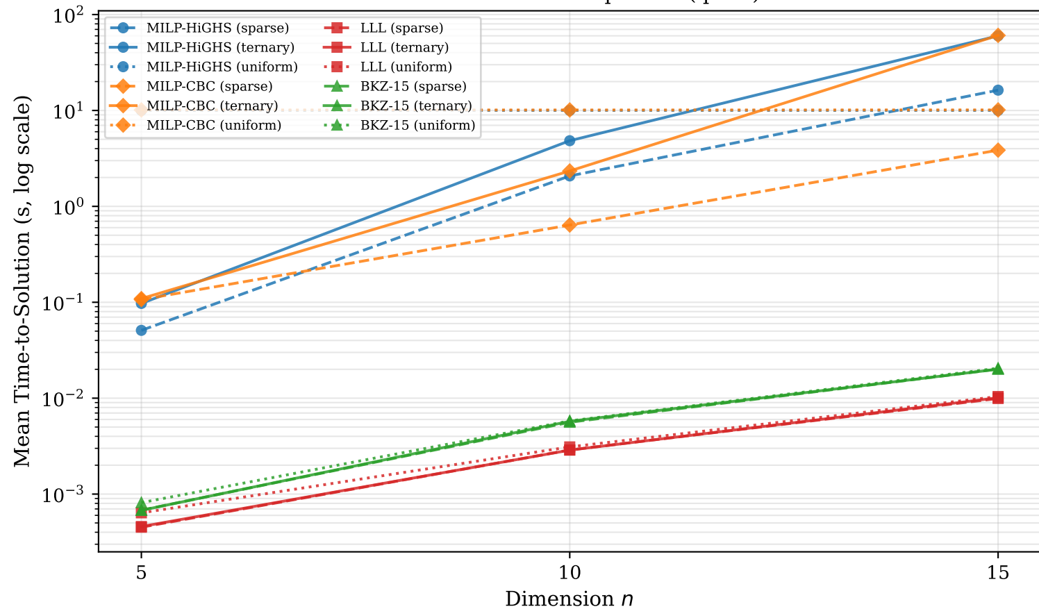
Time-to-Solution Comparison ( q=97 )
