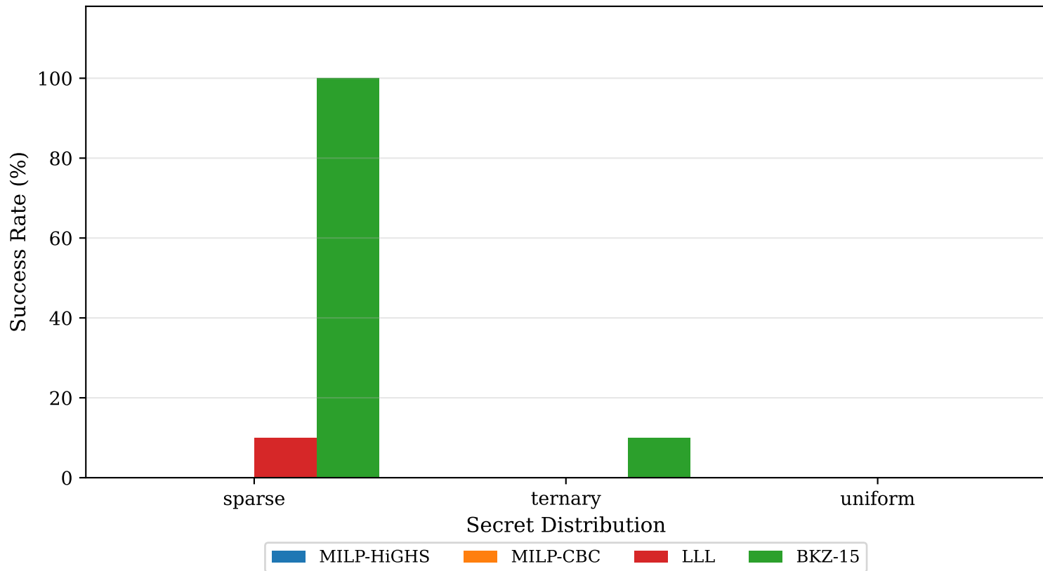
Success Rate by Secret Type at n = 50
