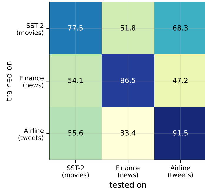
Tiny-BERT (+MLM pre-training)
