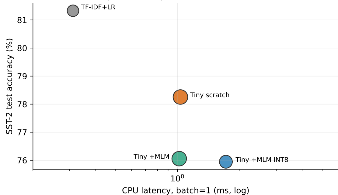
Accuracy vs latency (marker area ~ model size)
