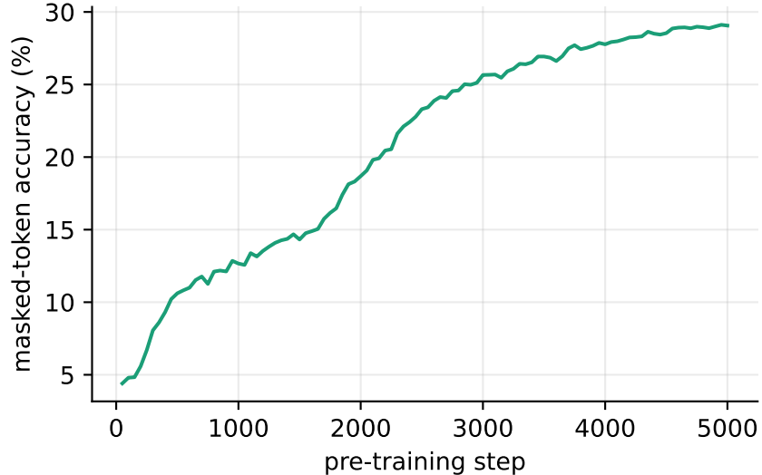
Held-out masked-token accuracy
