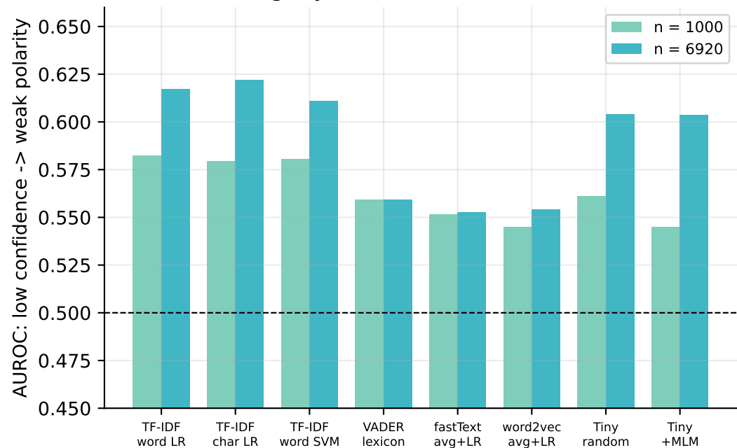
Ambiguity-awareness (0.5 = chance)
