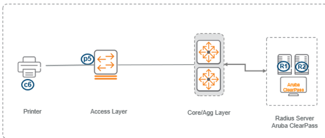
Figure 5 MAC authentication
