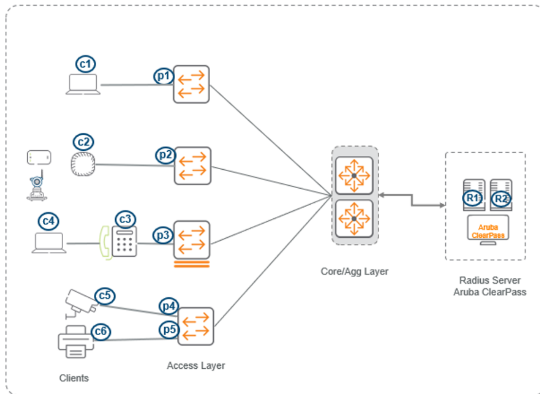
Figure 4 802.1X and MAC authentication
