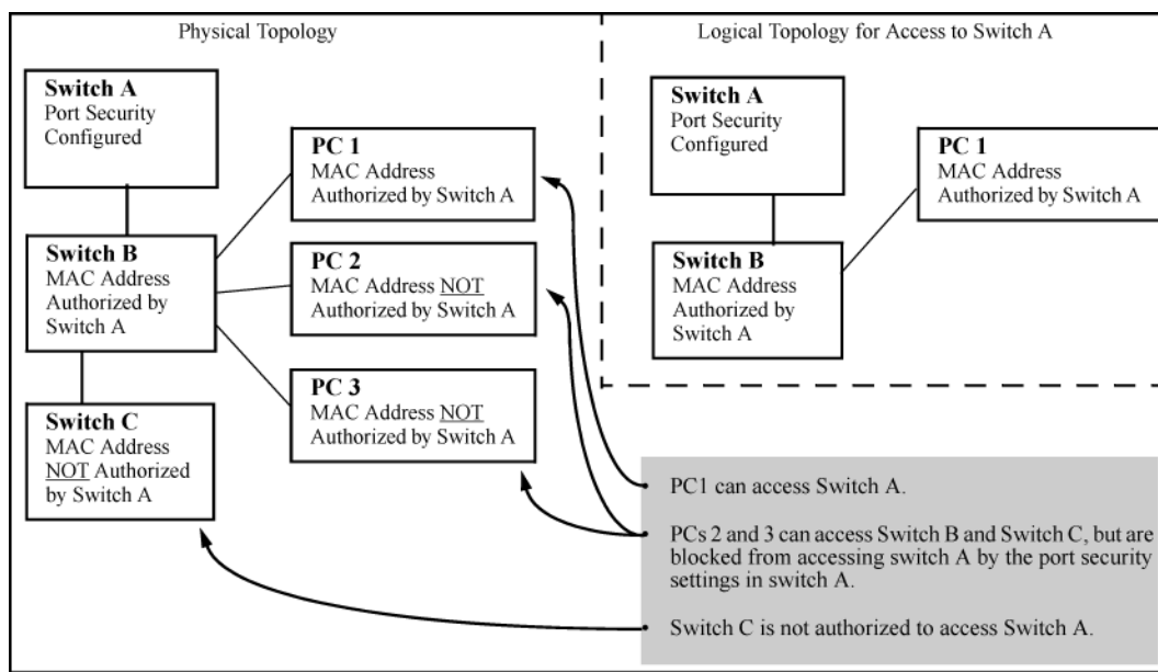
Figure 6 How port security controls access
