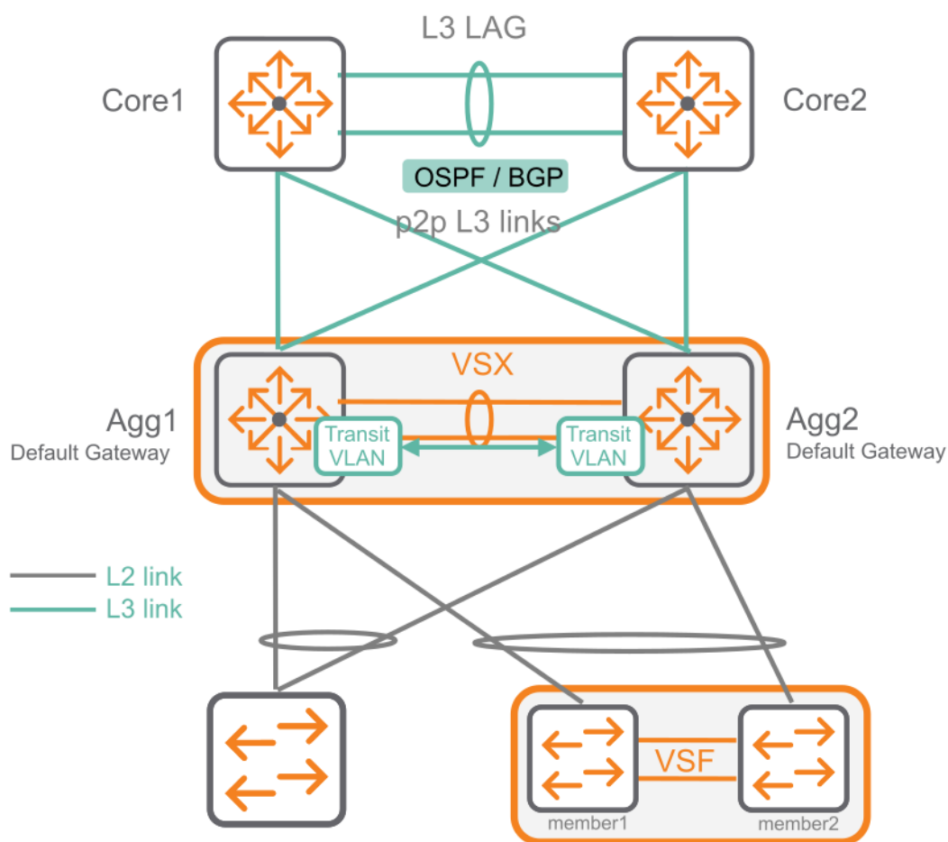
Figure 1 ROP with a single VRF in the VSX environment
