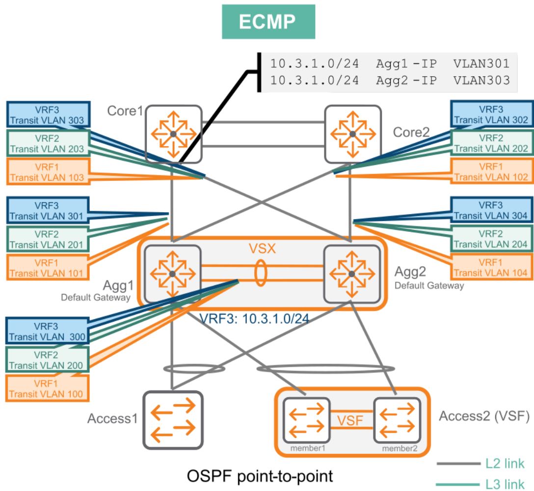
Figure 1 ECMP and VSX LAG in a VSX environment
