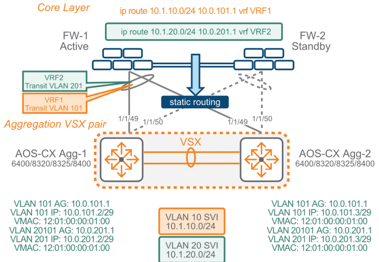
Figure 3 Active gateway as a next-hop router
