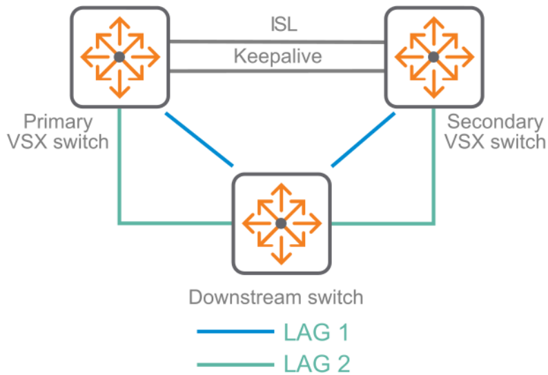
Figure 1 Example of Loop Protect Over VSX
