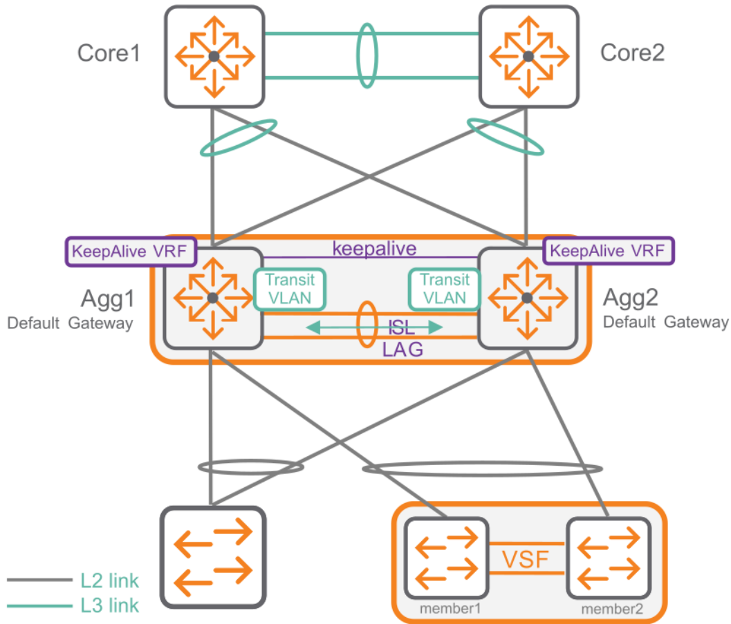
Figure 1 Recommended configuration for keepalive
