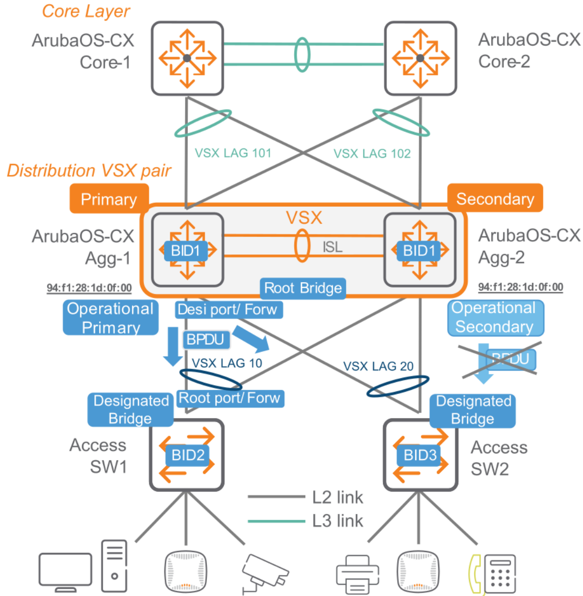
Figure 1 Sample MST on VSX configuration
