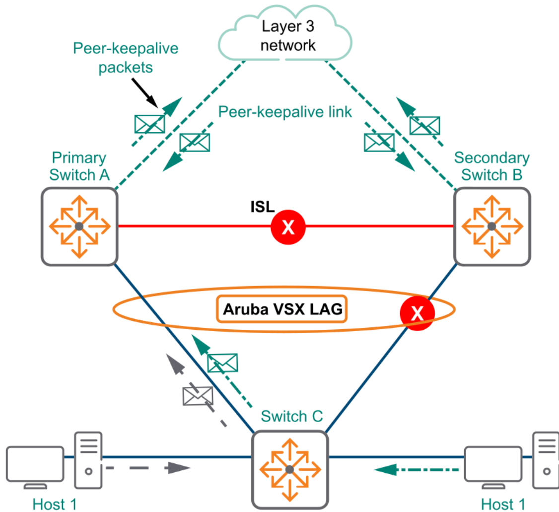
Figure 1 Keepalive topology
