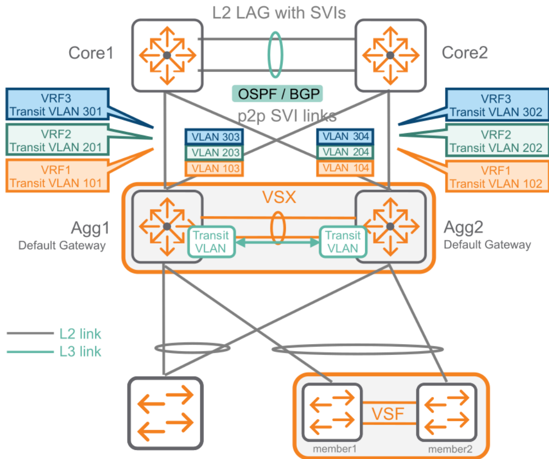
Figure 2 SVI (multiple VRFs) in a VSX environment
