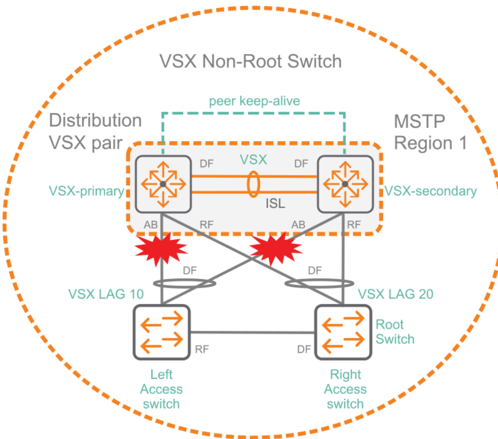
Figure 2 MSTP VSX pair as a nonroot switch
