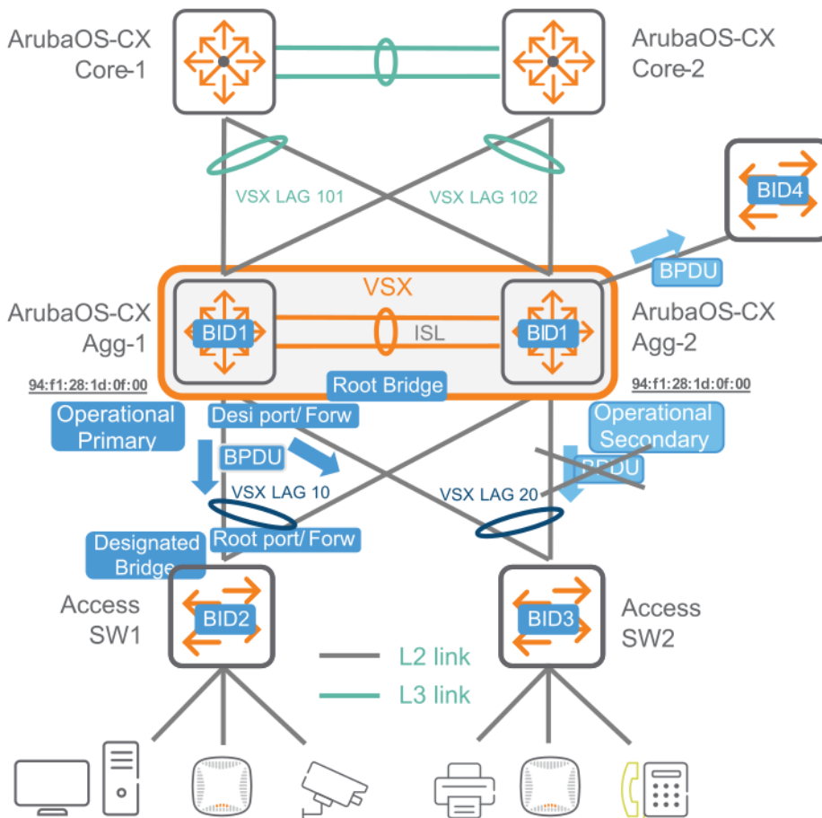
Figure 1 Physical view of the VSX and MSTP loop-protect configurations
