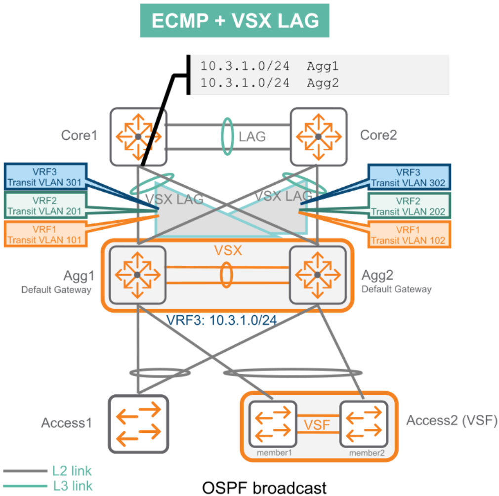
Figure 2 ECMP in a VSX environment
