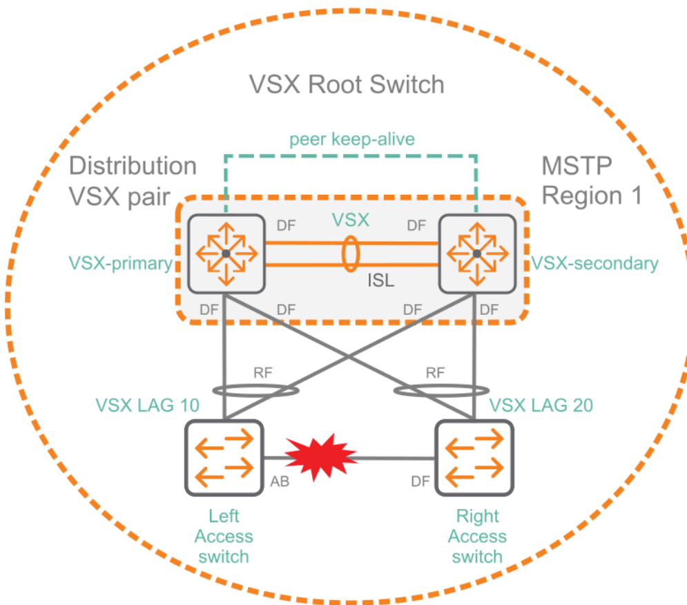
Figure 1 MSTP VSX pair as a root switch
