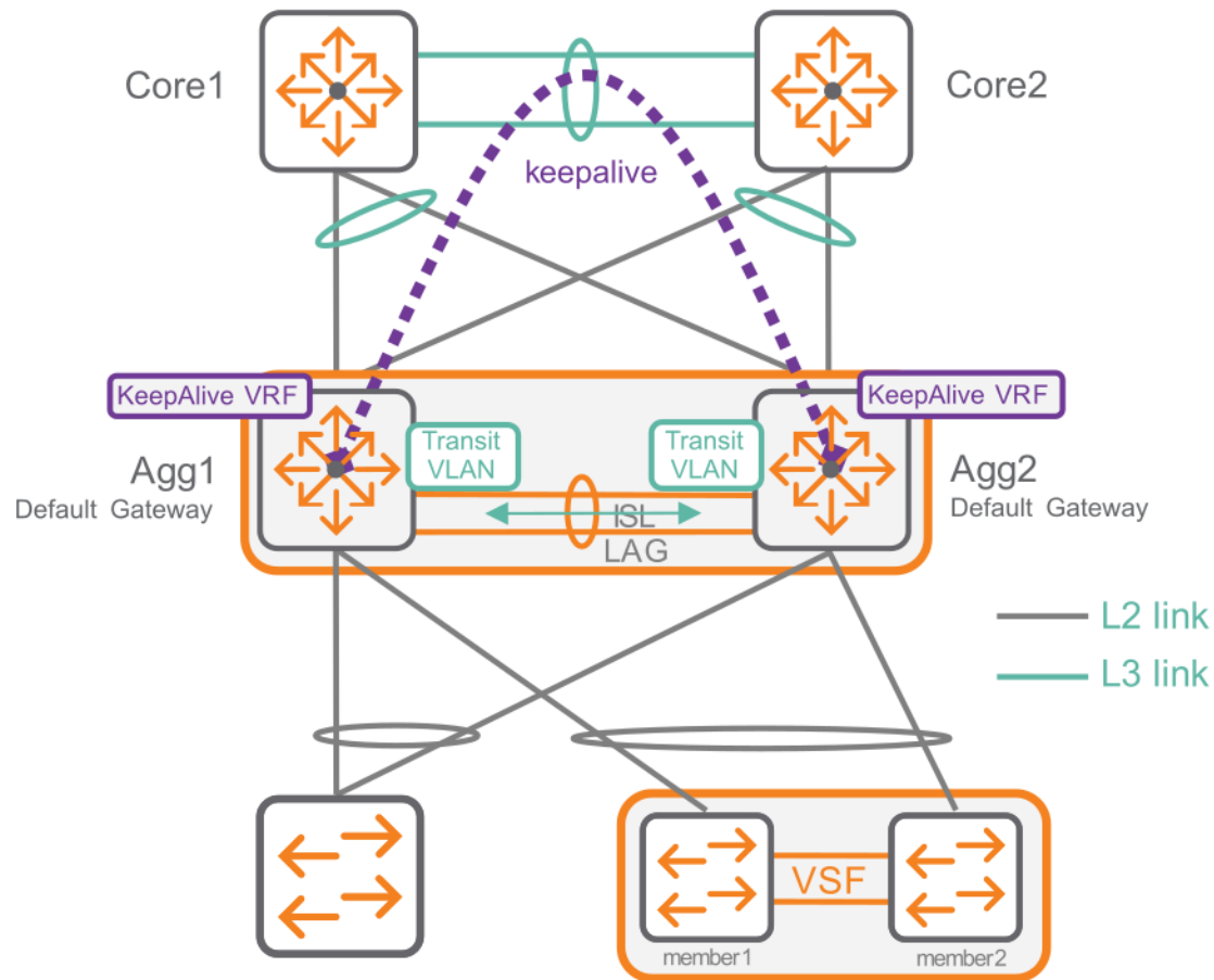
Figure 2 Not supported configuration for keepalive
