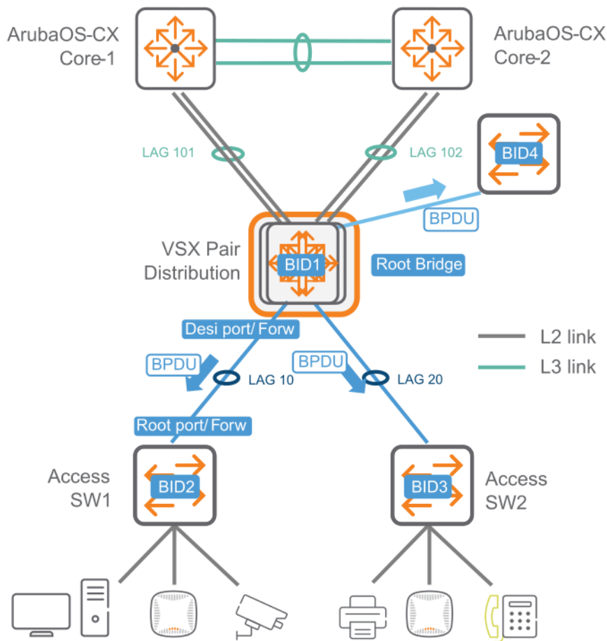
Figure 2 Logical view of the VSX and MSTP loop-protect configurations
