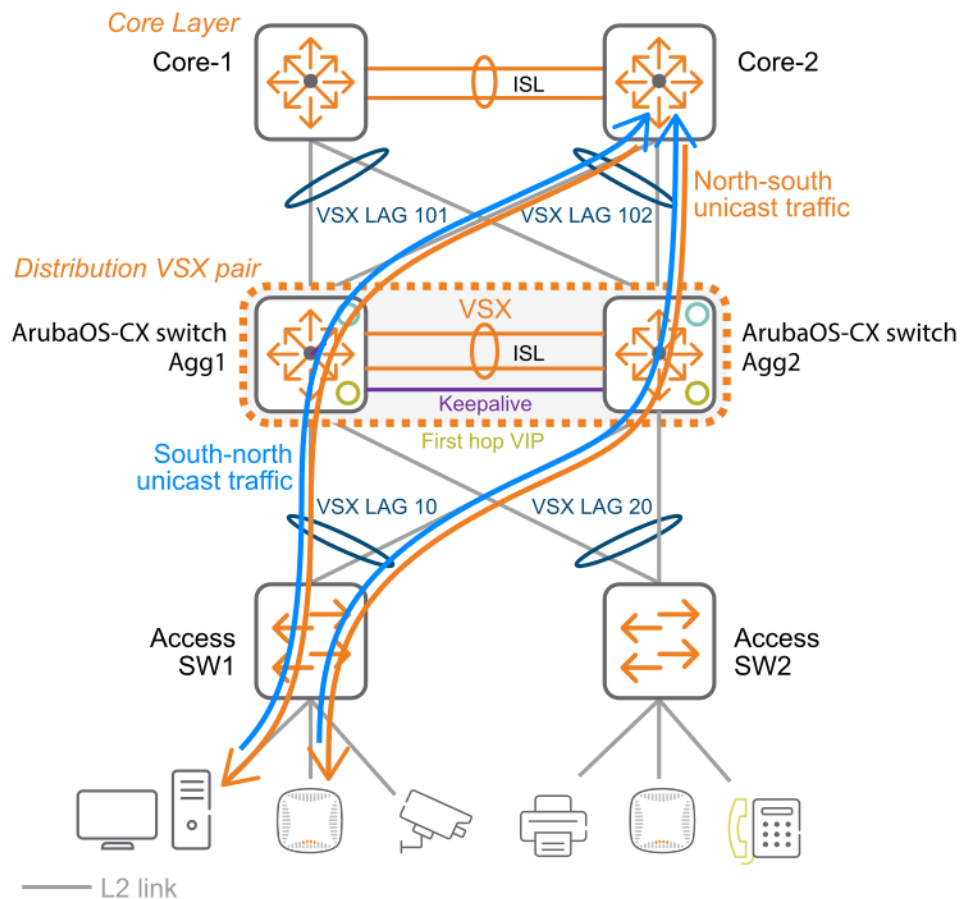
Figure 1 Active Forwarding and Active Gateway example
