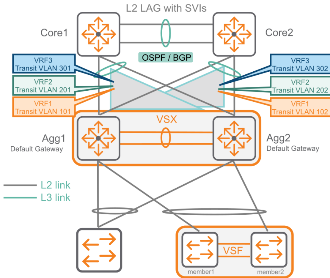
Figure 3 VSX LAG and layer 3 ECMP
