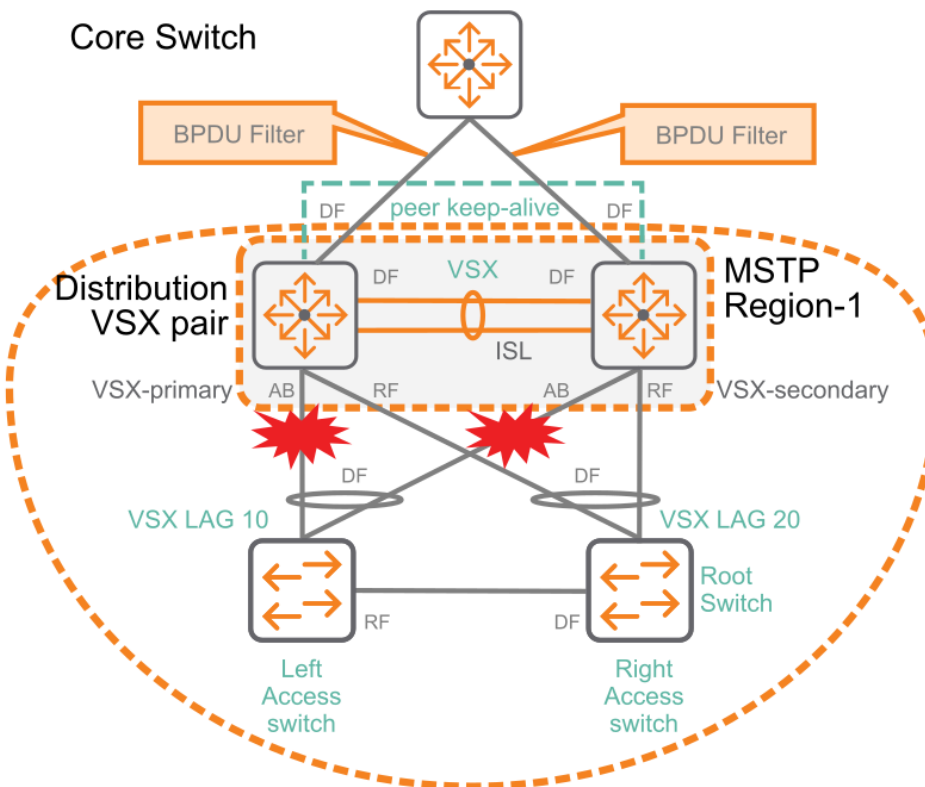
Figure 3 Distribution layer with VSX and MSTP connected to the core switch
