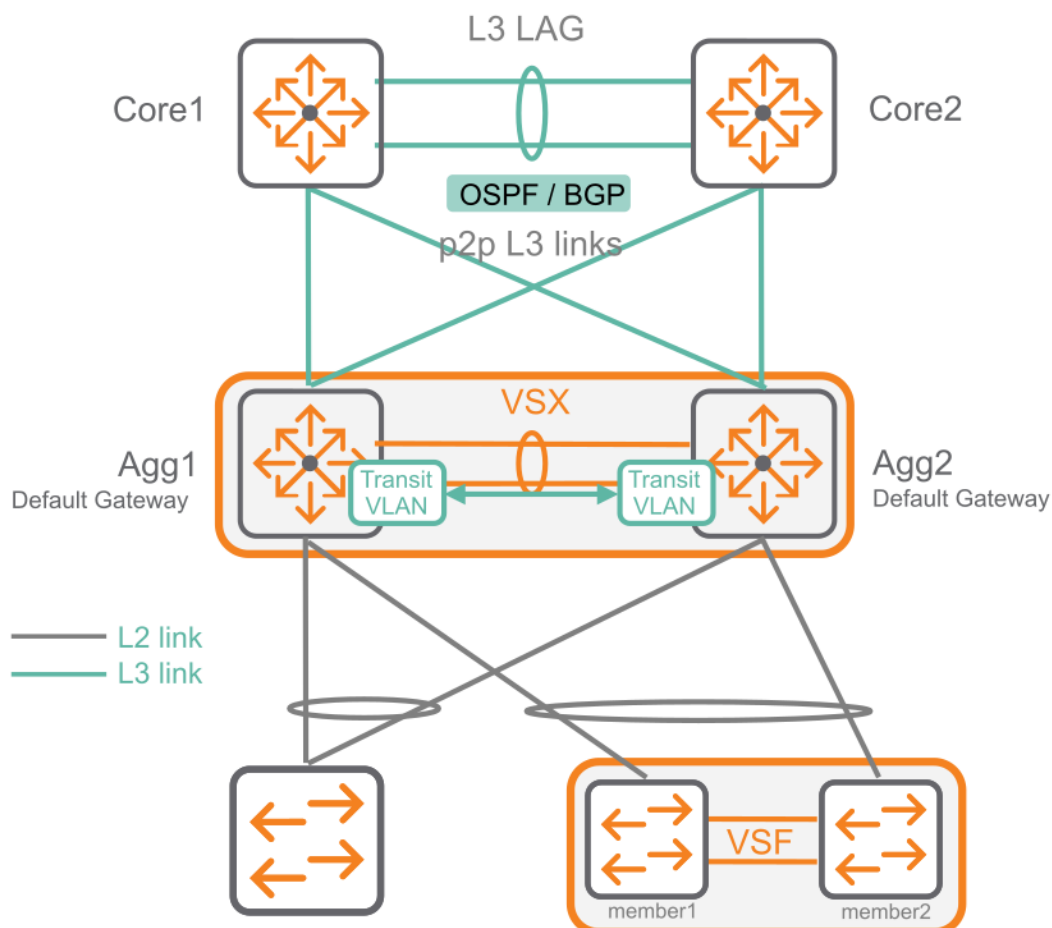
Figure 1 ROP with a single VRF in the VSX environment
