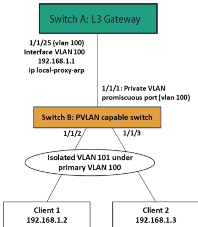
Figure 1 Local Proxy ARP Use Case Example
