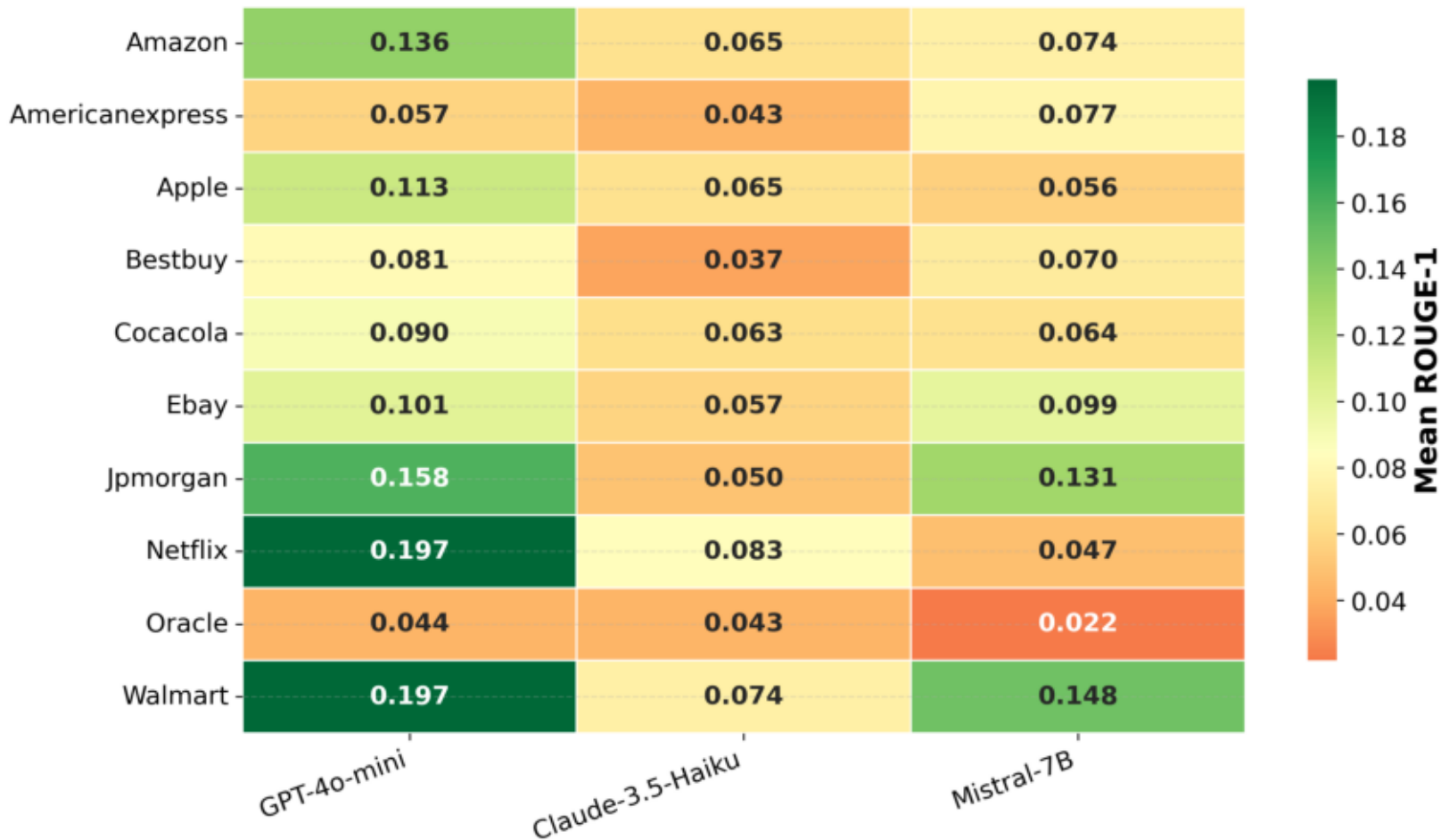
Per-Company ROUGE-1 Heatmap (Fine-tuned embeddings, temp=0.0, k=5)
