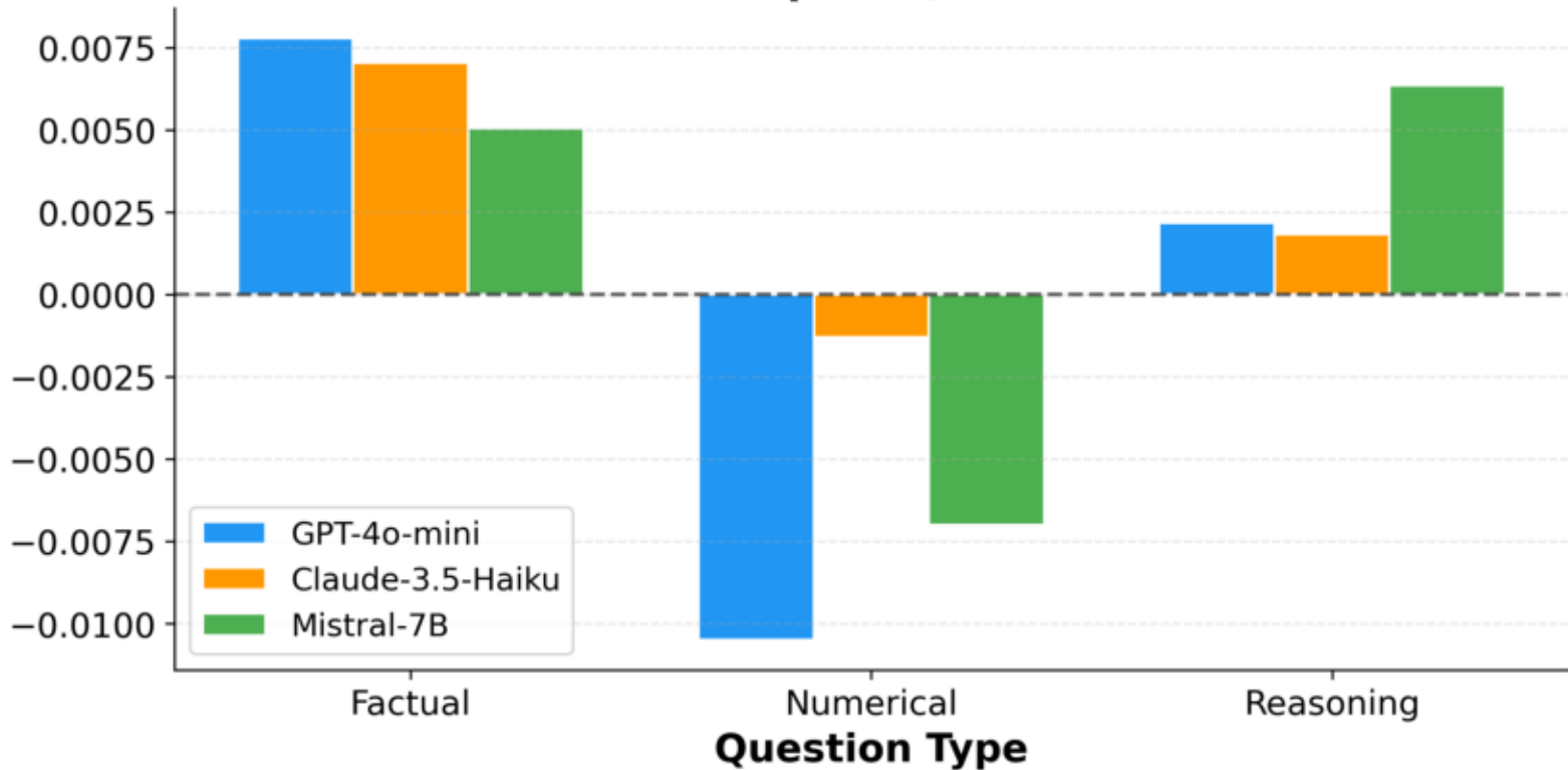
Fine-tuning Delta by Question Type (temp=0.0, k=5)
