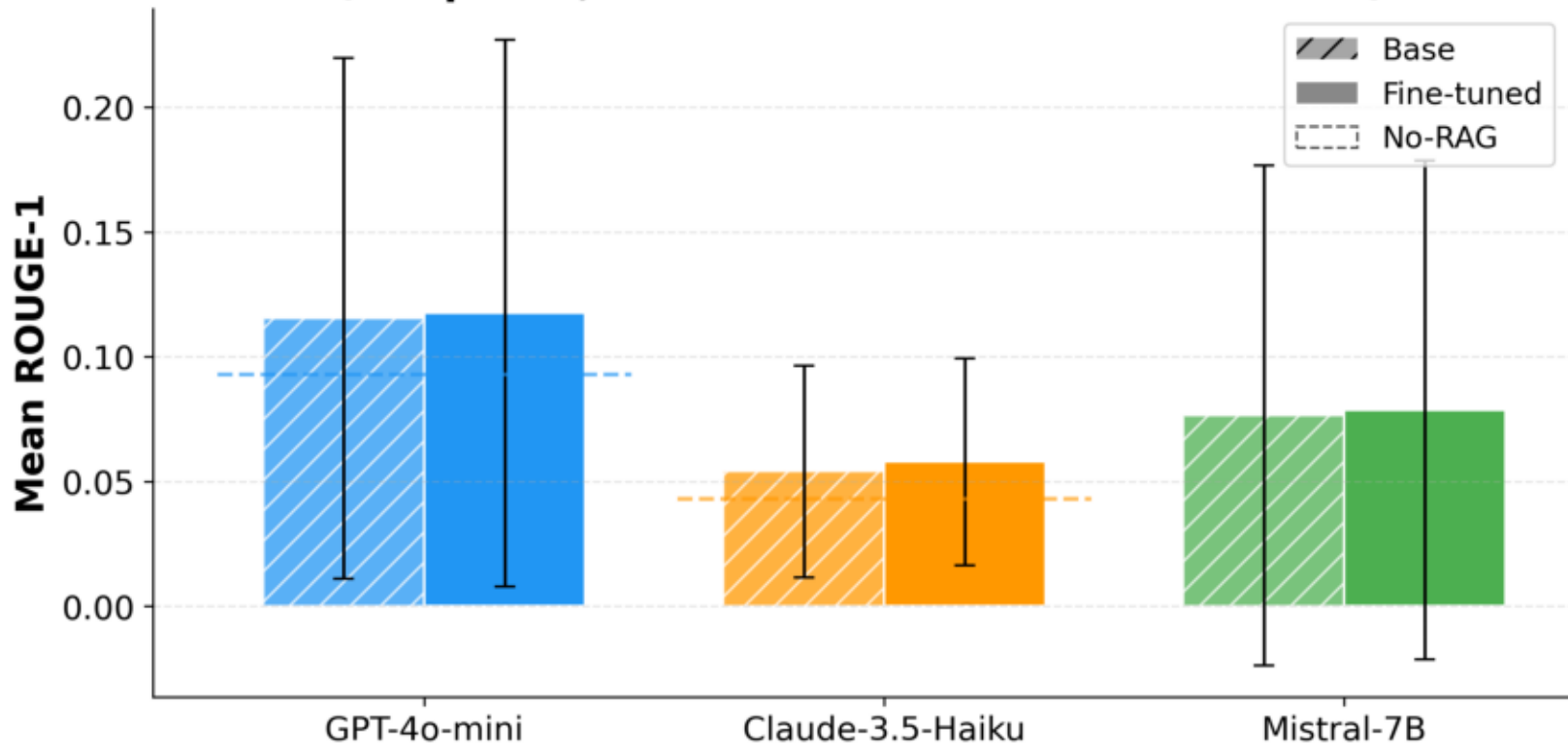
ROUGE-1 by Model and Embedding Type (temp=0.0, k=5 — dashed = no-RAG baseline)
