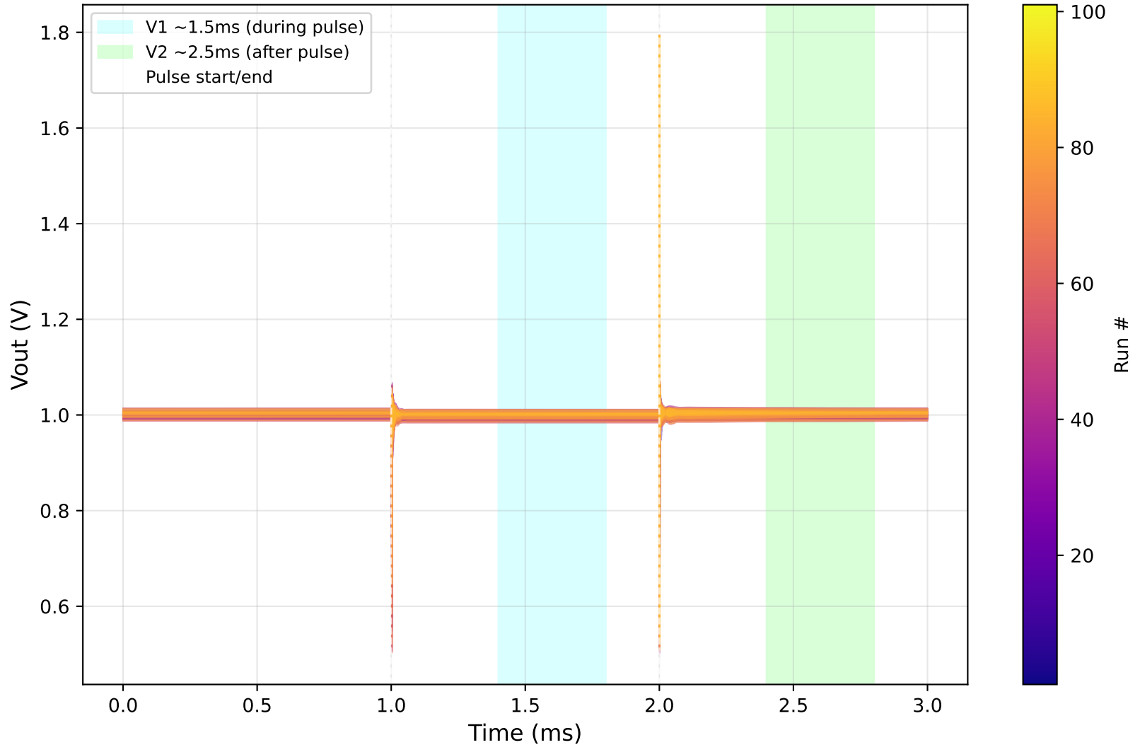
Monte Carlo - Load Regulation (101 runs)
