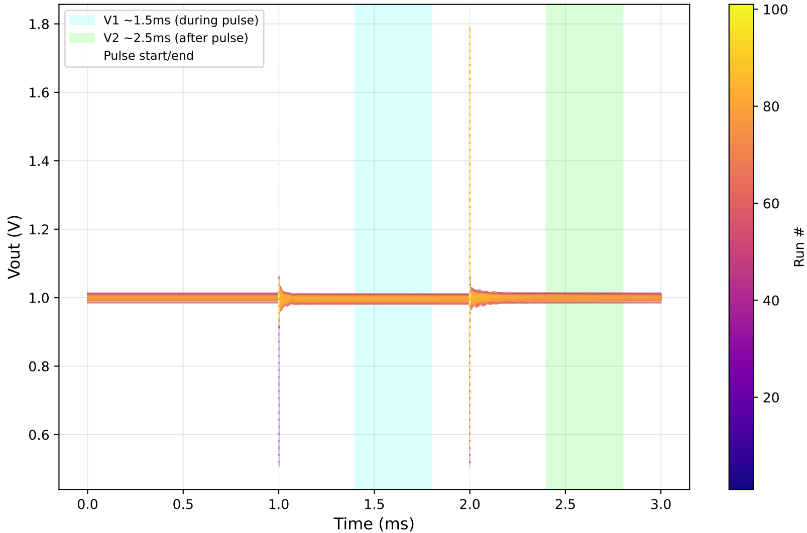
Monte Carlo - Load Regulation (101 runs)
