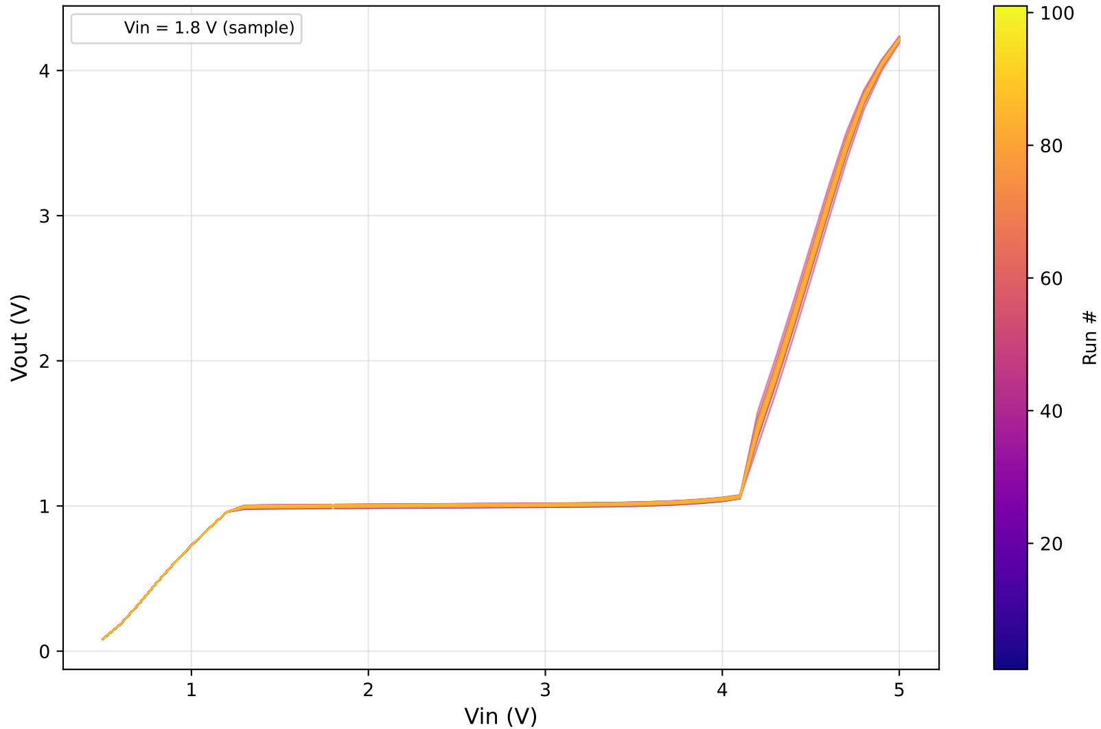
Monte Carlo - Vout vs Vin (101 runs)
