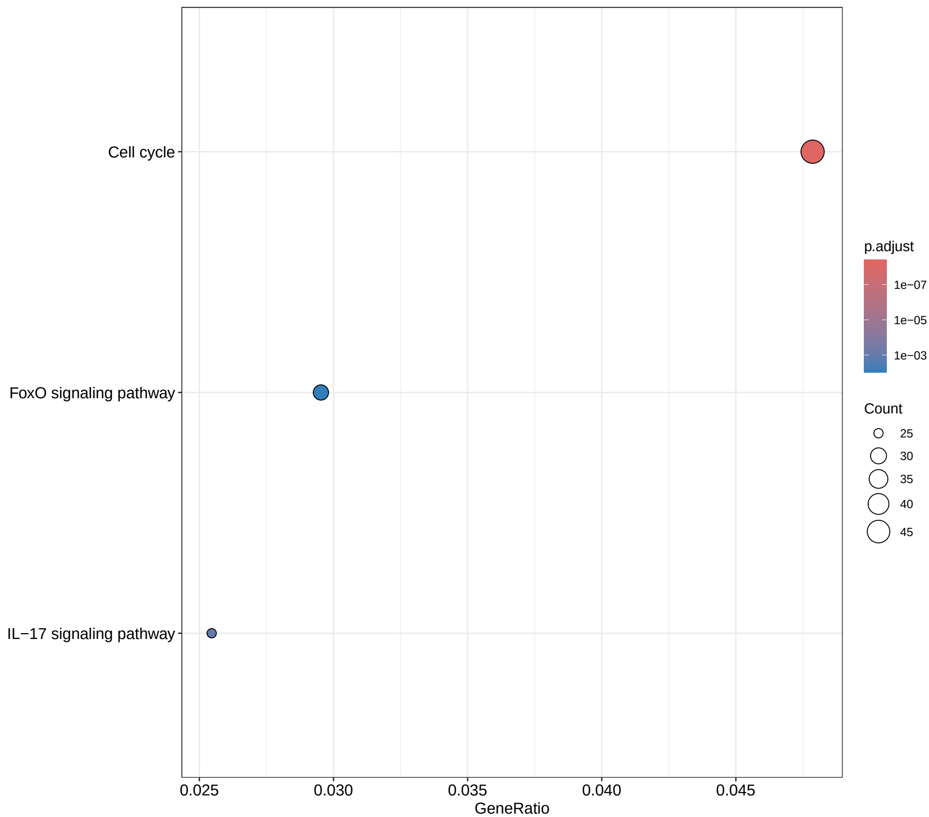
KEGG Pathways — NSCLC DEGs
