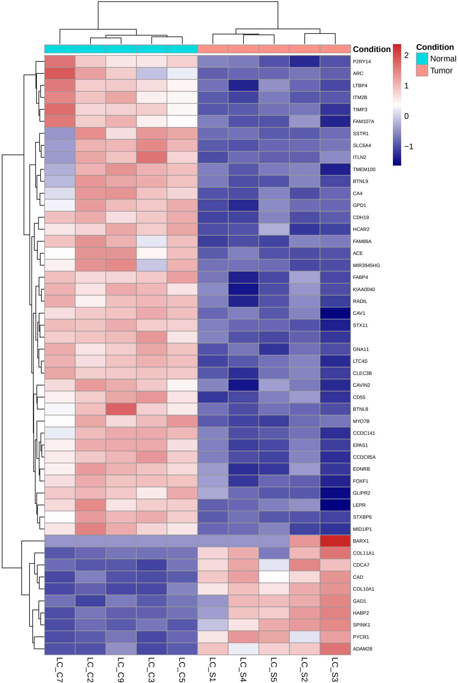
Top 50 DEGs — NSCLC Tumor vs Normal (GSE40419)
