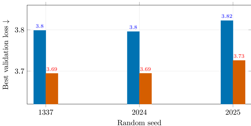
AdamW Hybrid Muon 125M Fineweb-Edu: AdamW vs Hybrid Muon
