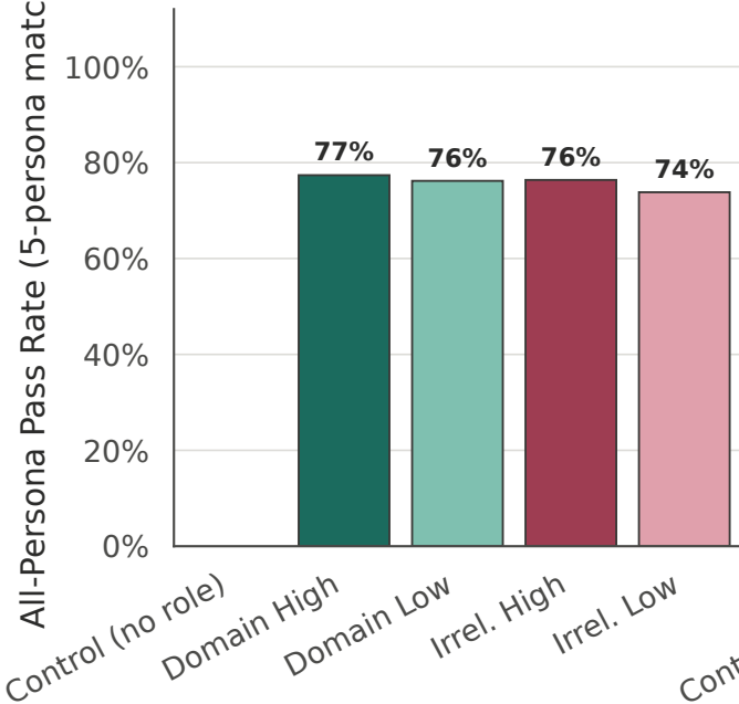
Qwen3-8B (thinking)
