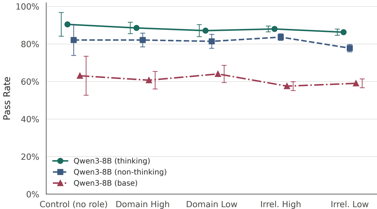
Pass Rate by condition, per model
