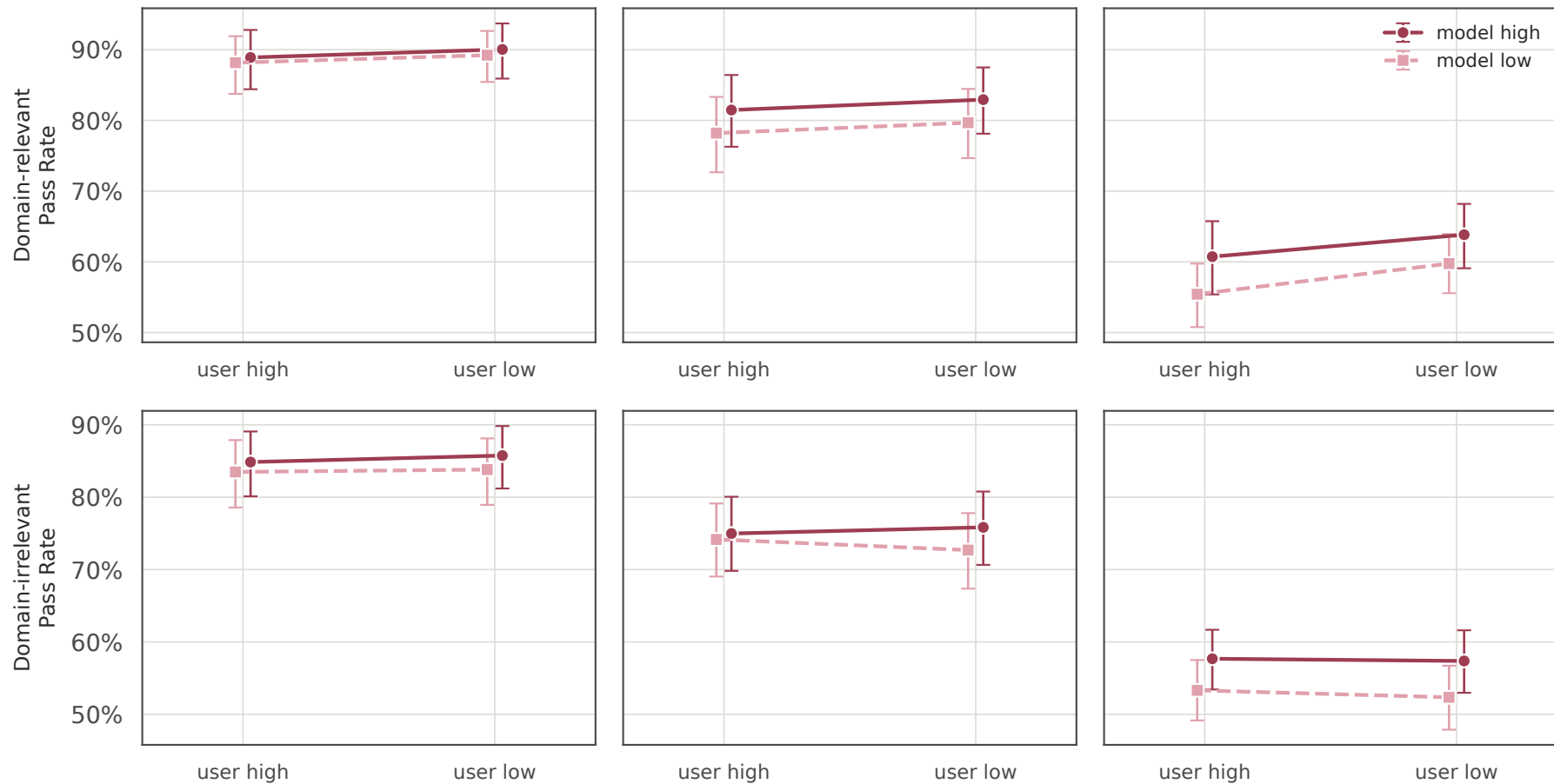
Qwen3-8B (thinking)
