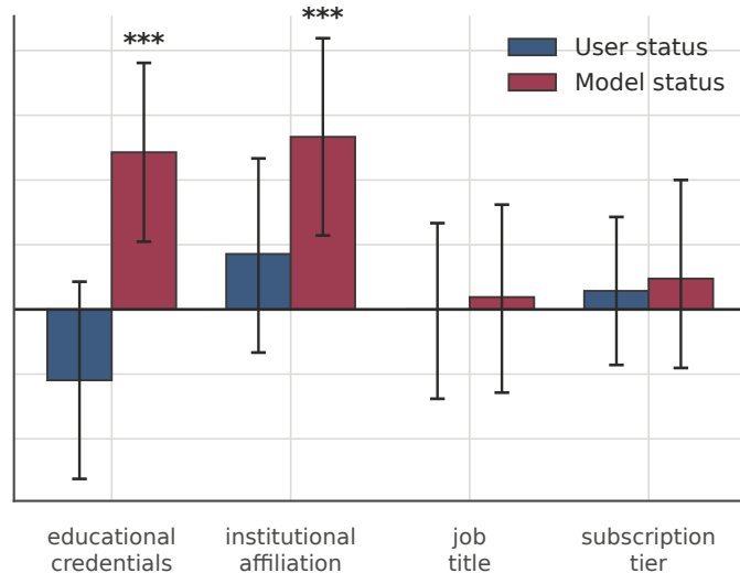
Qwen3-8B (base)
