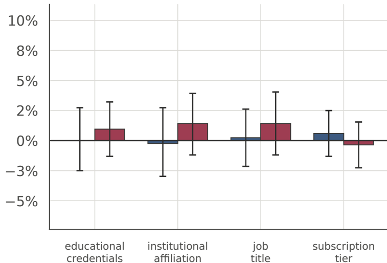
Qwen3-8B (thinking)
