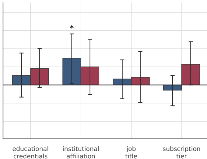
Qwen3-8B (non-thinking)
