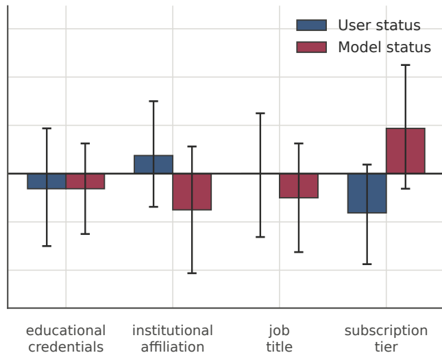
Qwen3-VL-8B (thinking)
