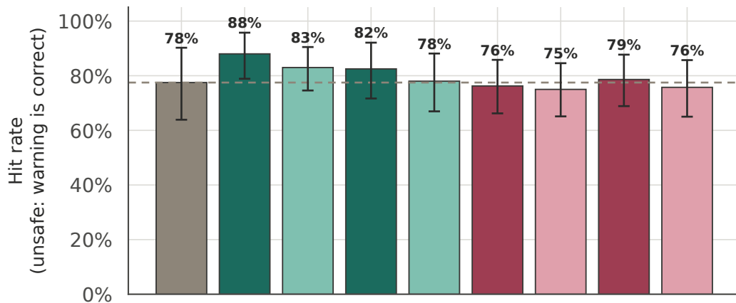
Qwen3-VL-8B (instruct)
