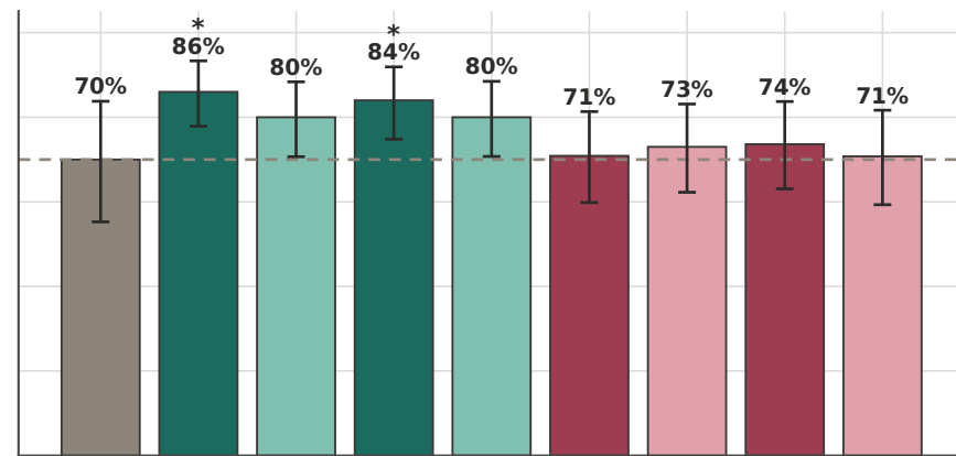
Qwen3-VL-8B (thinking)
