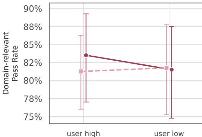
Qwen3-VL-8B (instruct)
