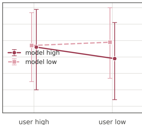
Qwen3-VL-8B (thinking)
