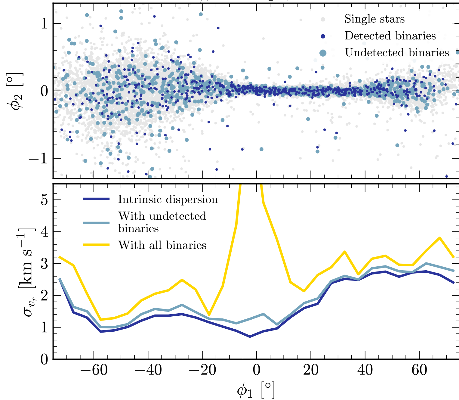
R_{\text{vir},0} = 0.75 \text{ pc} ; lo-OB
