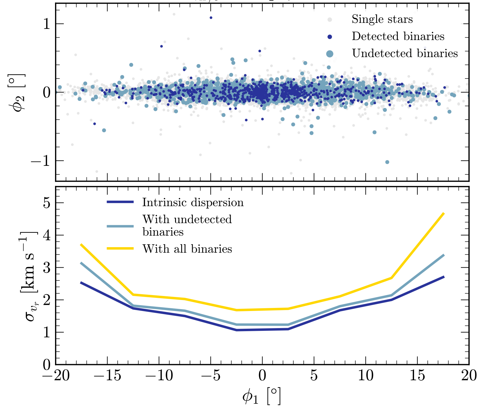
R_{\text{vir},0} = 6.0 \text{ pc} ; hi-OB
