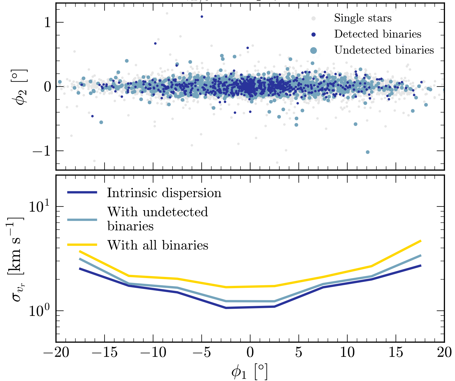
R_{\text{vir},0} = 6.0 pc; hi-OB
