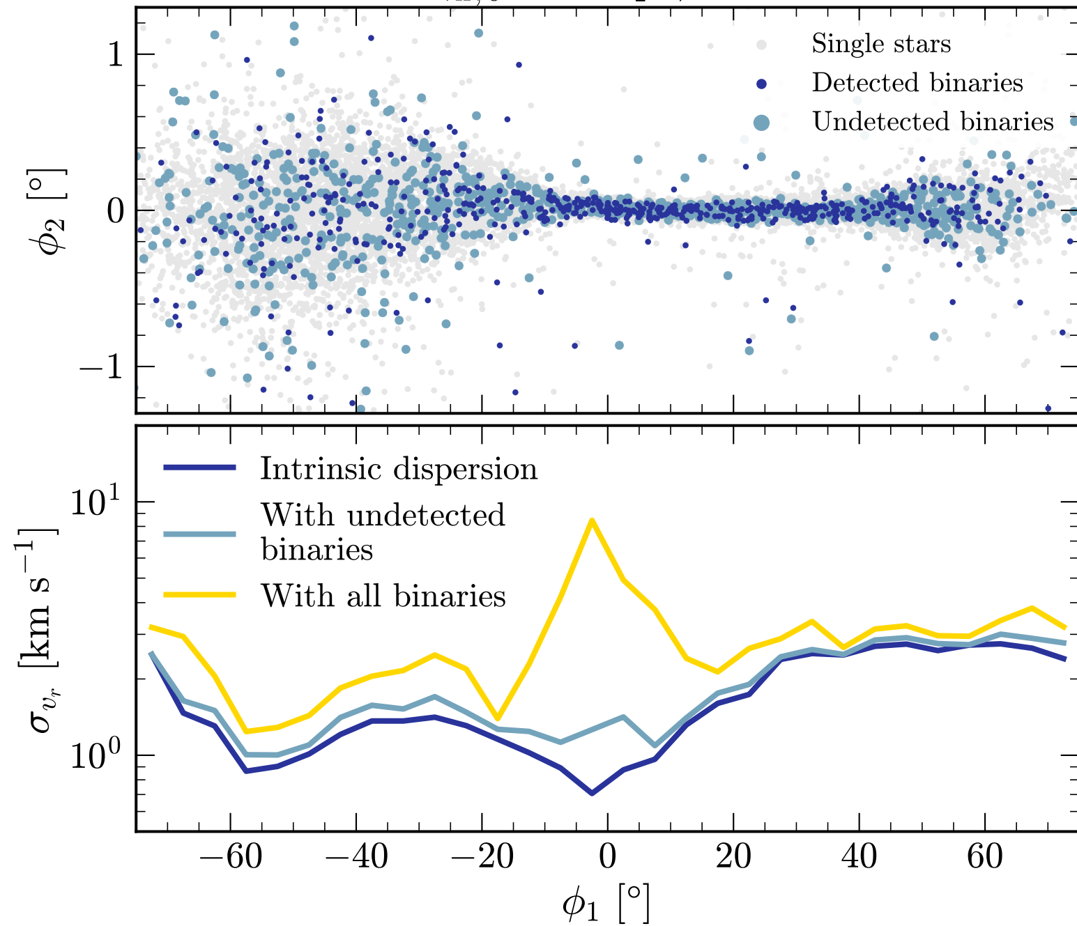
R_{\text{vir},0} = 0.75 pc; lo-OB
