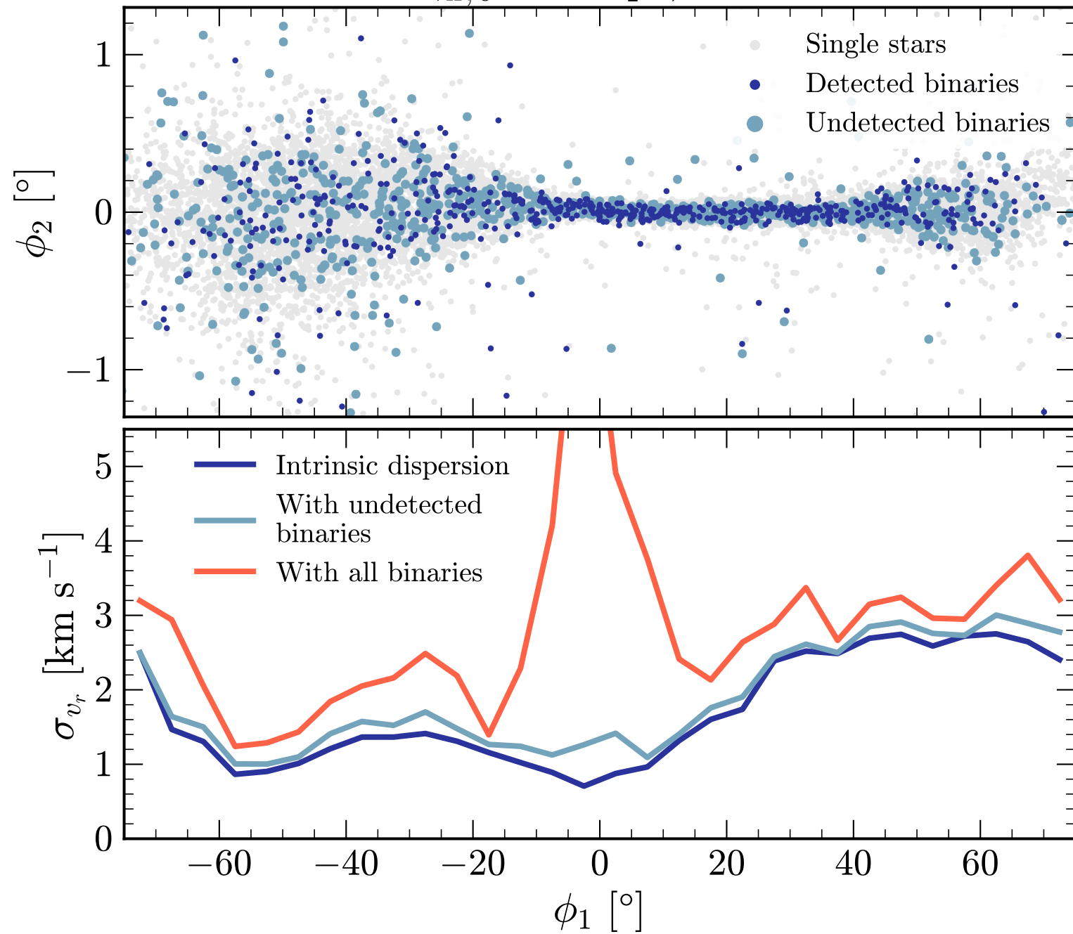
R_{\text{vir},0} = 0.75 pc; lo-OB
