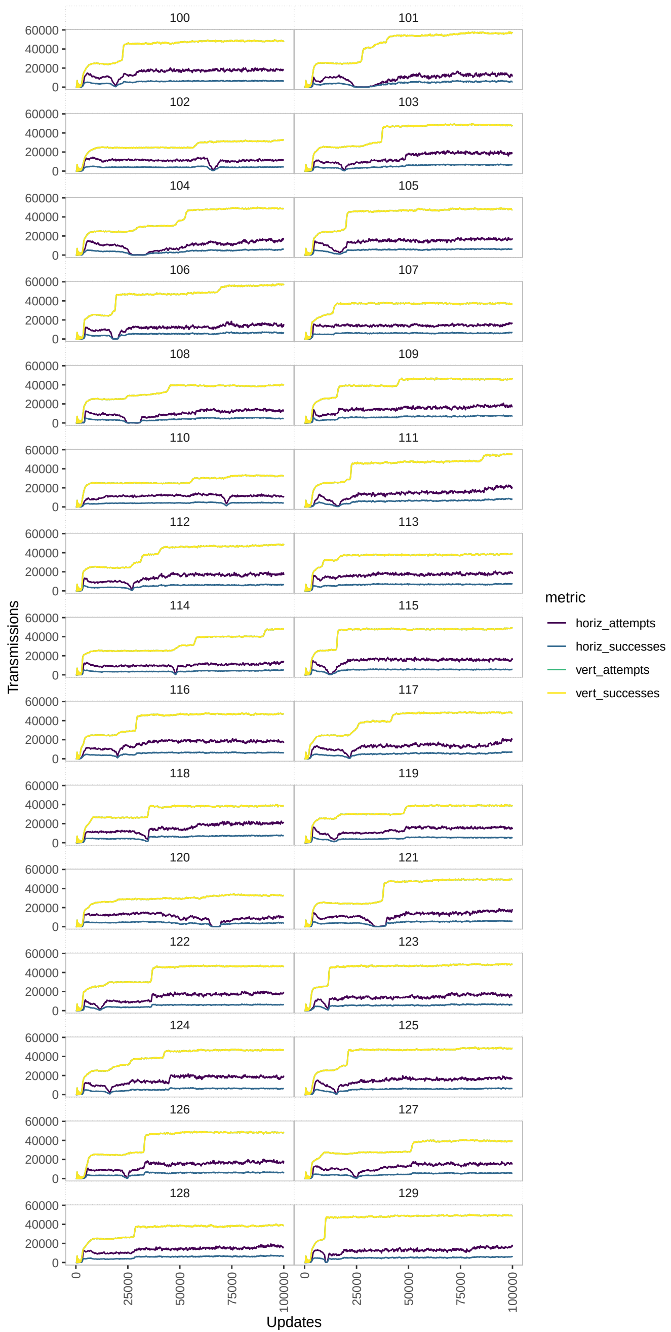
mutualists-mixed
