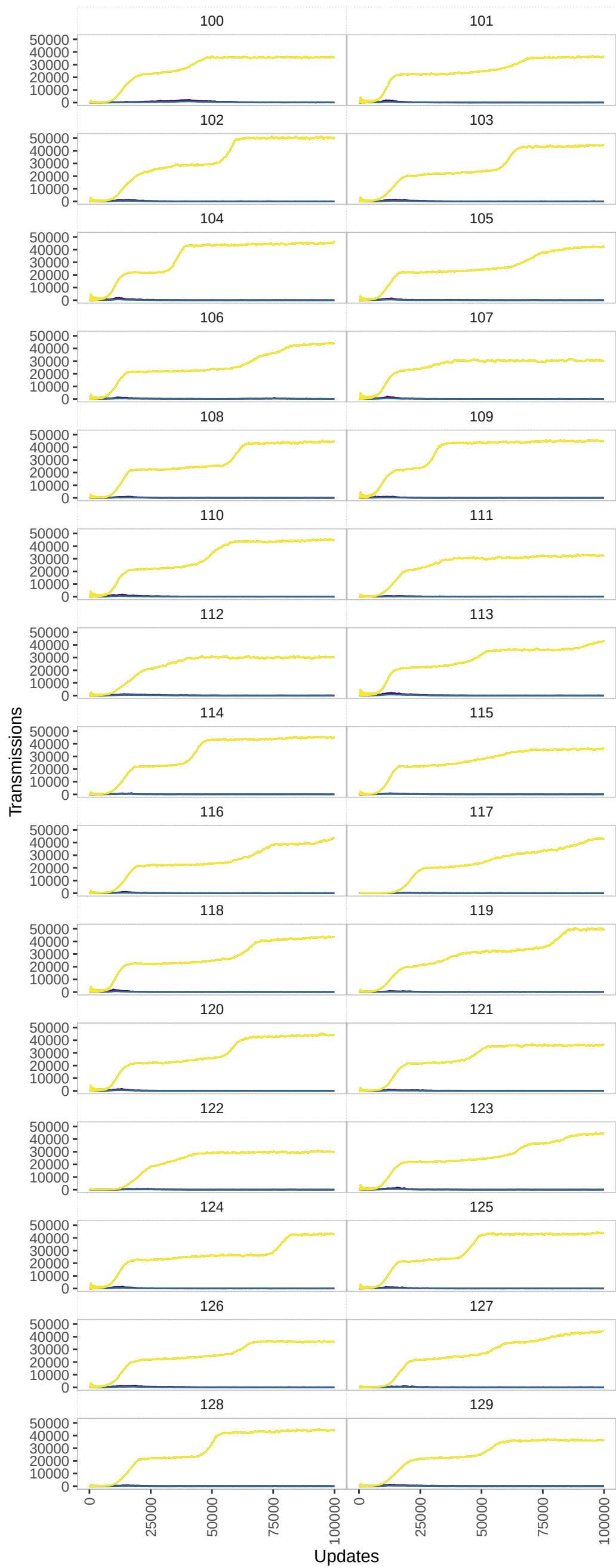
mutualists-grid
