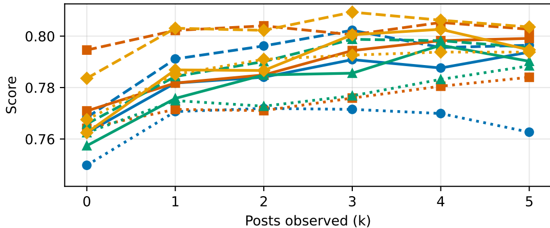
Accuracy
