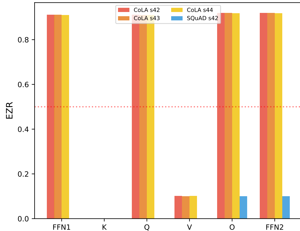
(a) EZR at Layer 11
