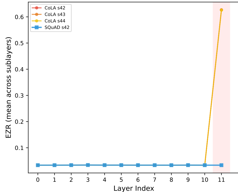
(c) Layerwise EZR — Seed Consistency
