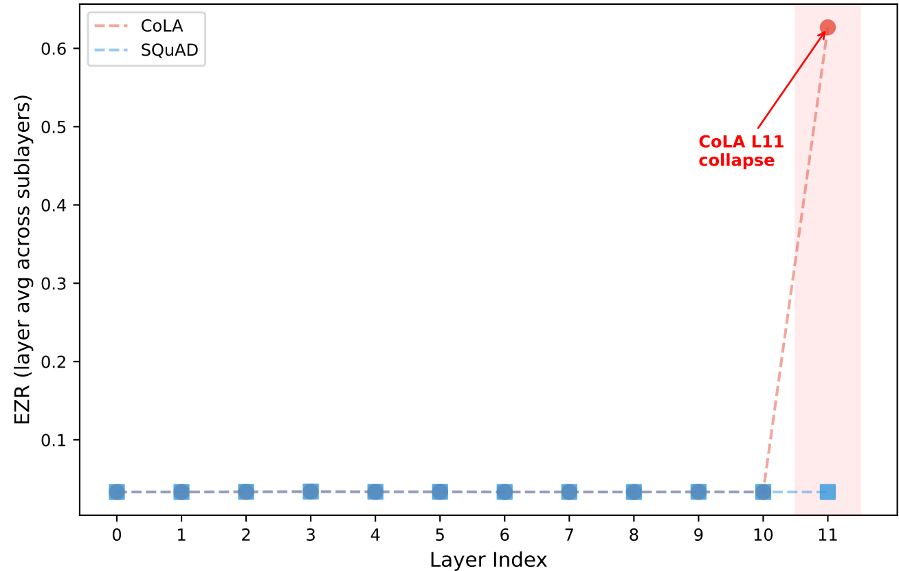
(c) EZR by Layer — L11 Collapse in CoLA
