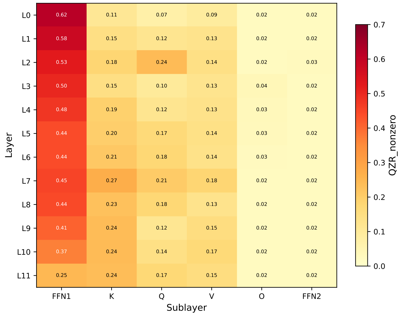
SQuAD
